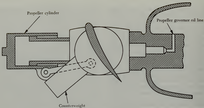
FIGURE 7-11. Pitch change mechanism for a counterweight propeller.
